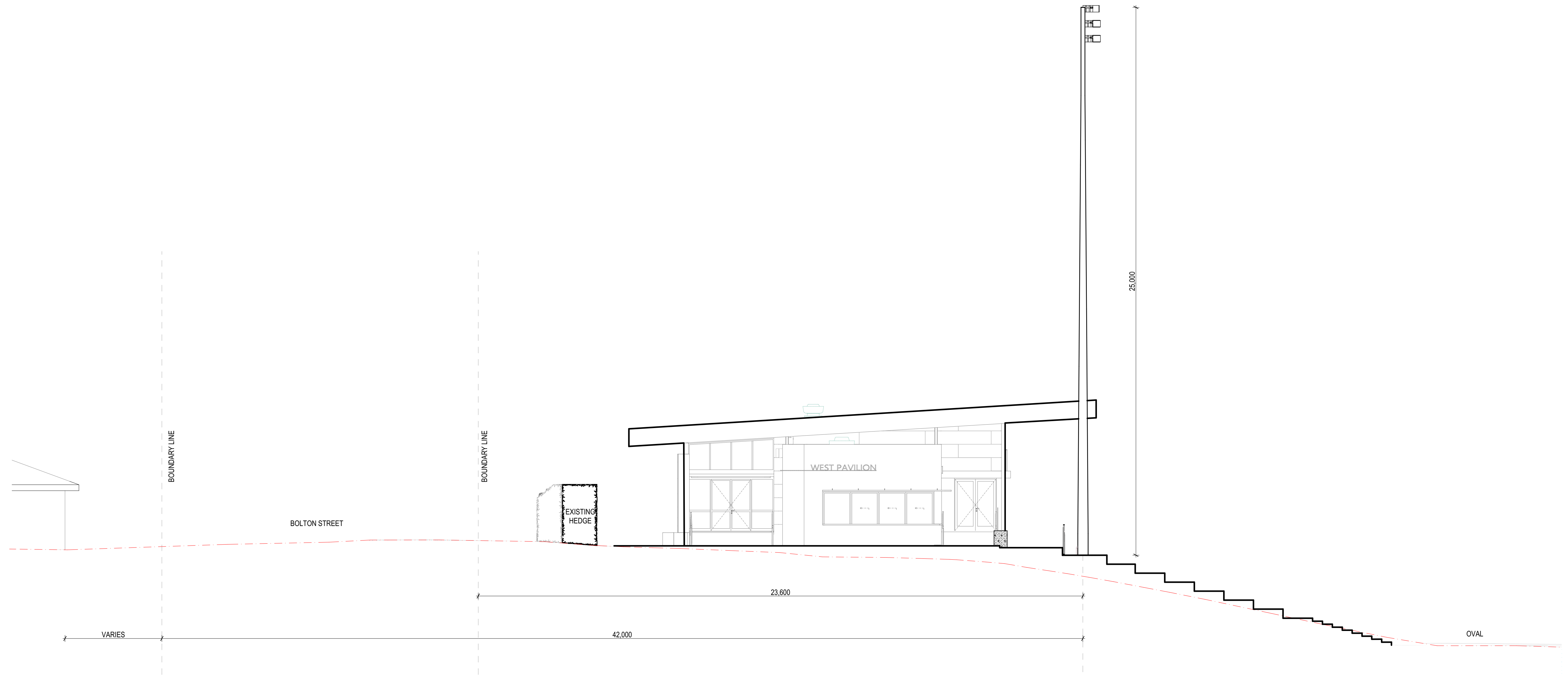
○ OVAL LIGHTING TOWER 1 SECTION
